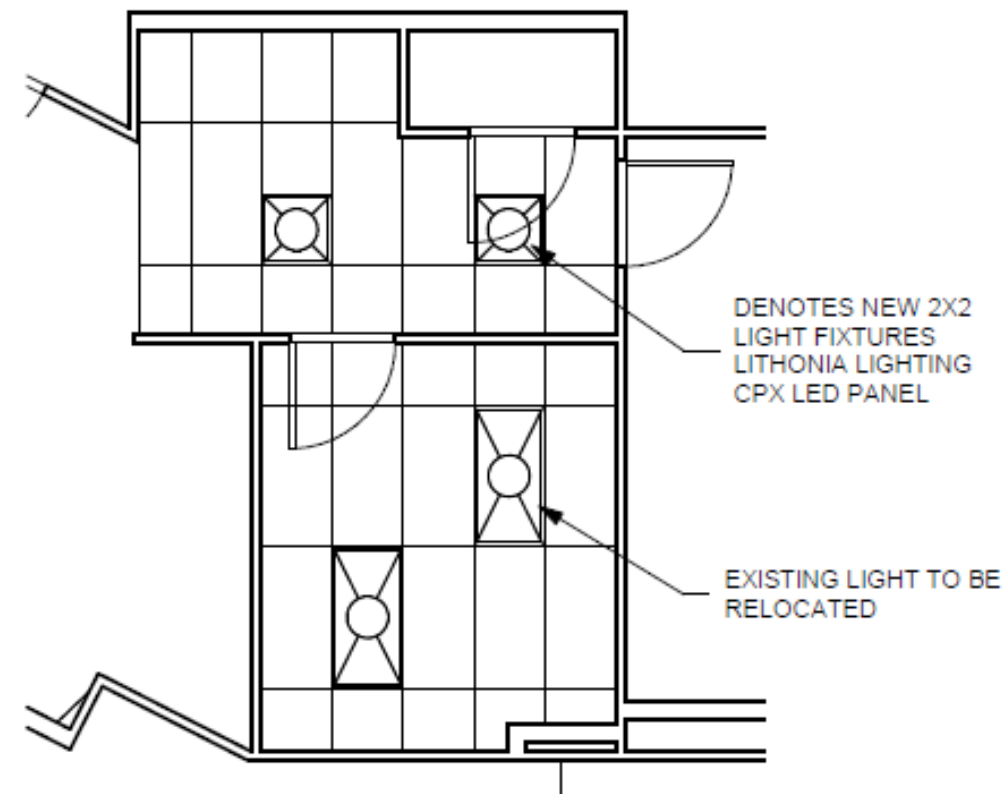
③ CEILING PLAN 3/16" = 1'-0"
