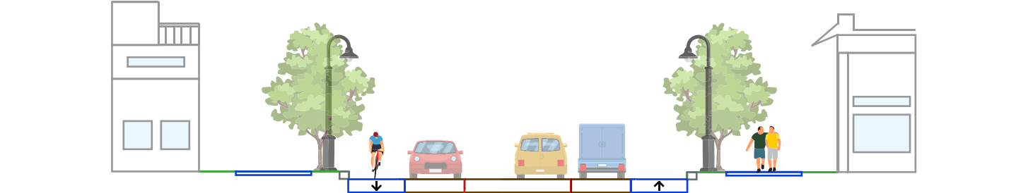
FIGURE 4.14 - STREET SECTION - LOCAL 2
