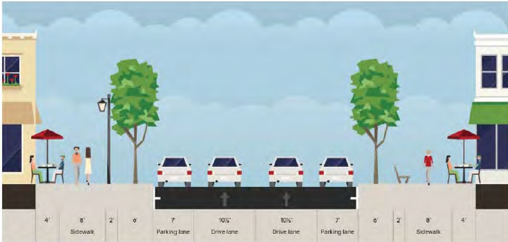
FIGURE 3.4 - CONCEPTUAL MAIN STREET SECTION
