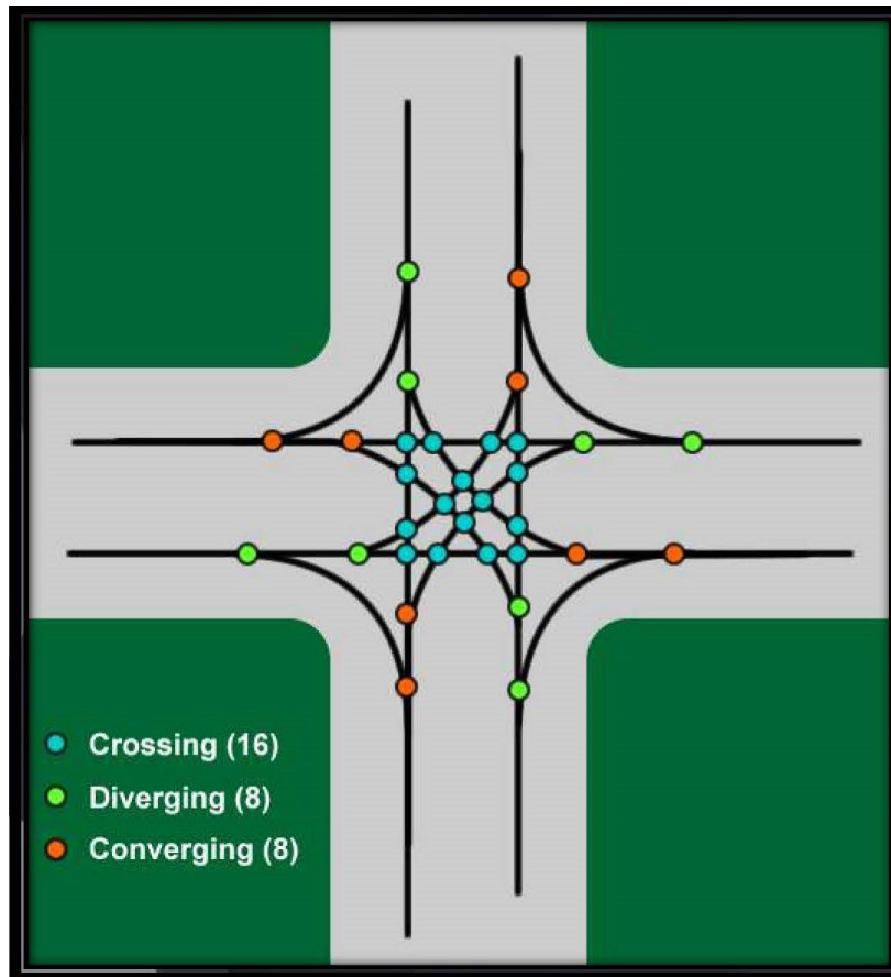
Traditional Intersection
